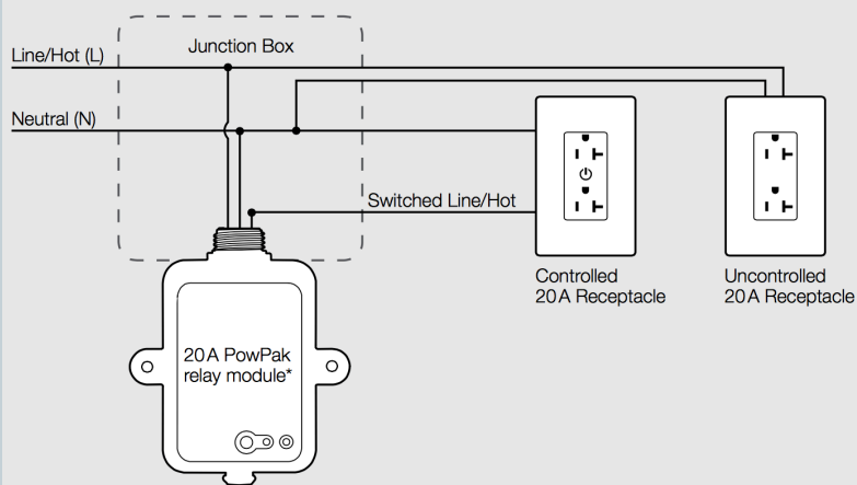
Diagram 2: Duplex Receptacle
